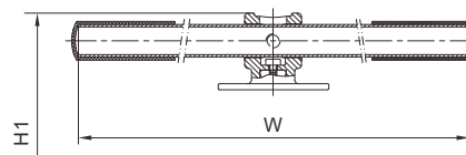
Gear Operation (Optional)
