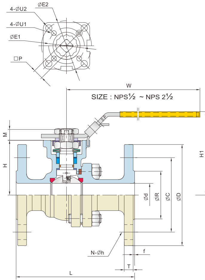
Direct Mount Pad (ISO 5211)
